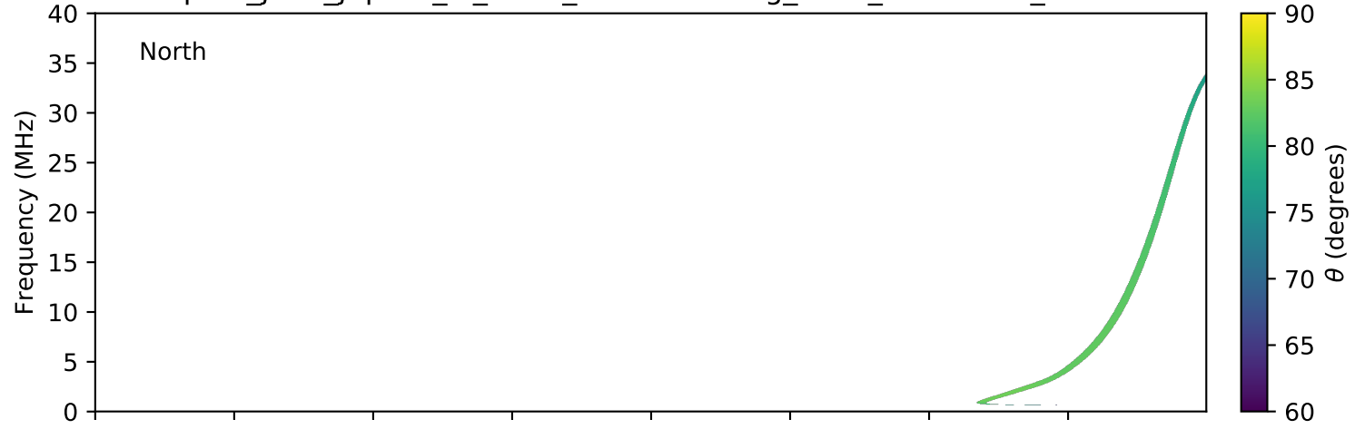
expres_juno_jupiter_io_isaac_lossc-wid1deg_3kev_20170405_v01.cdf
