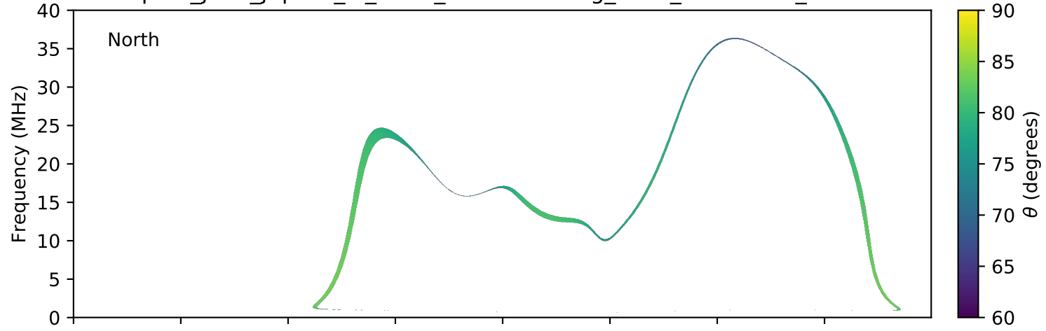
expres_juno_jupiter_io_isaac_lossc-wid1deg_3kev_20170402_v01.cdf
