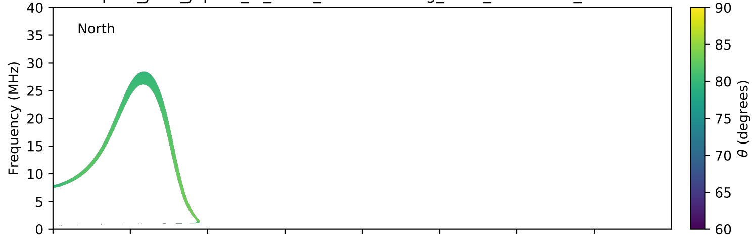
expres_juno_jupiter_io_isaac_lossc-wid1deg_3kev_20170401_v01.cdf
