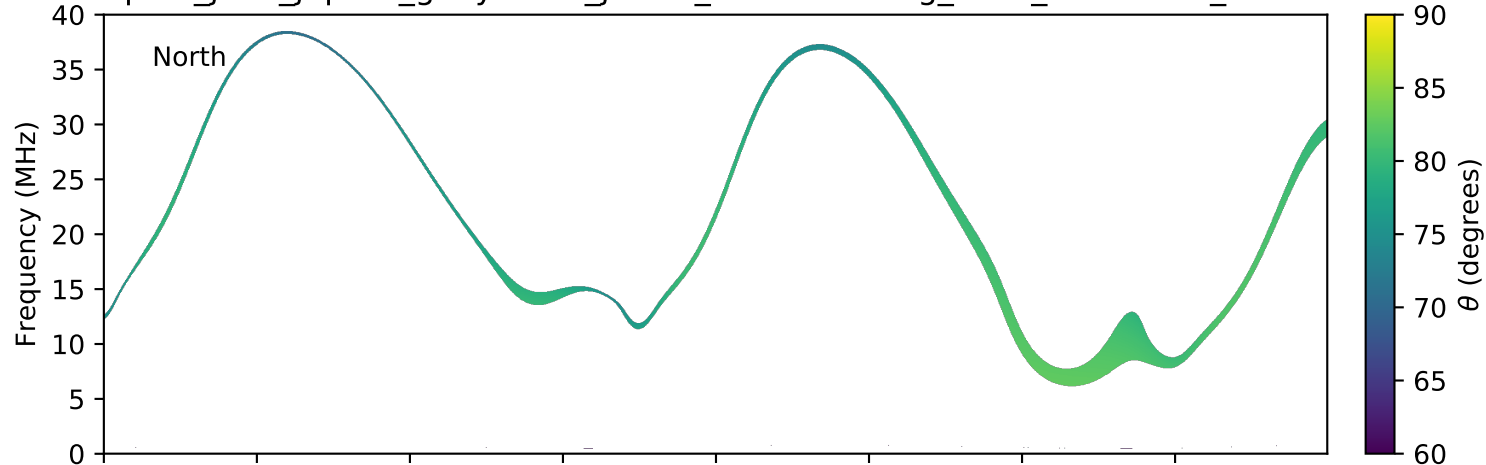
expres_juno_jupiter_ganymede_jrm09_lossc-wid1deg_3kev_20170420_v01.cdf
