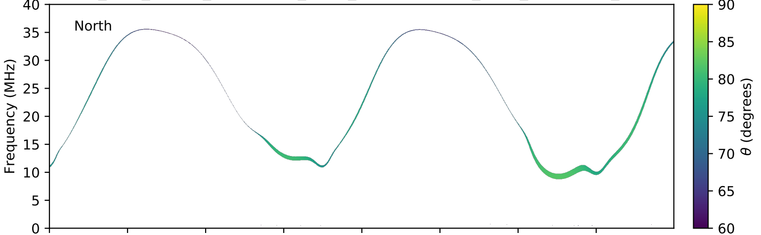
expres_juno_jupiter_ganymede_isaac_lossc-wid1deg_3kev_20170427_v01.cdf
