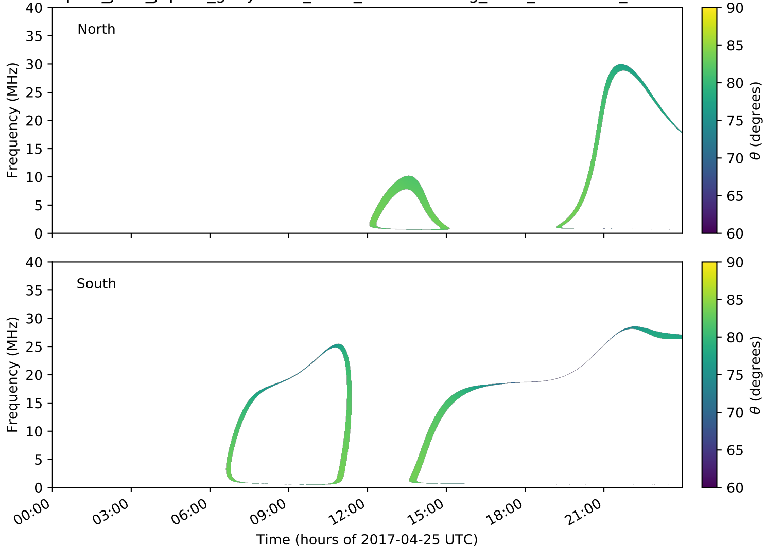
expres_juno_jupiter_ganymede_isaac_lossc-wid1deg_3kev_20170425_v01.cdf
