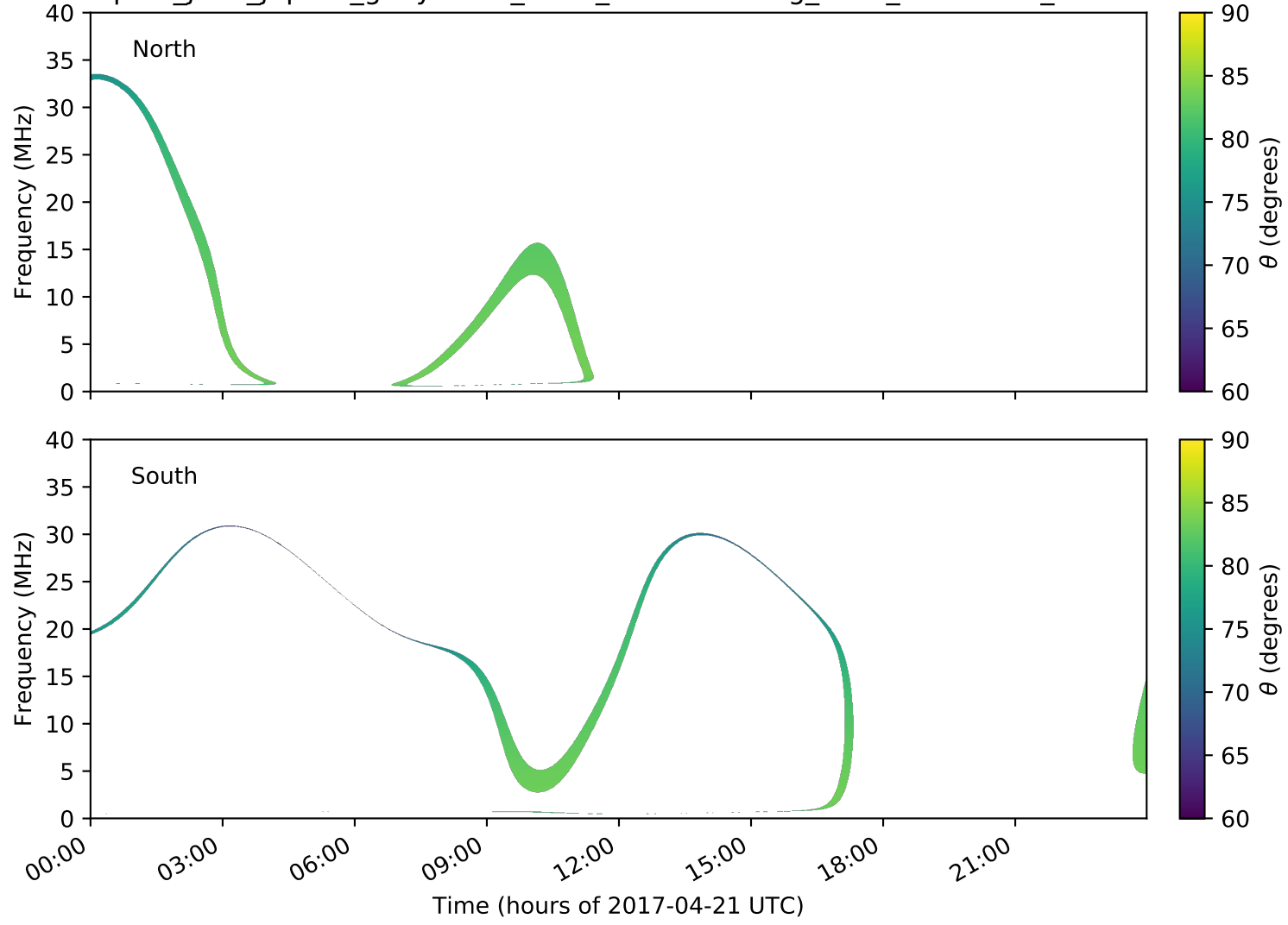
expres_juno_jupiter_ganymede_isaac_lossc-wid1deg_3kev_20170421_v01.cdf
