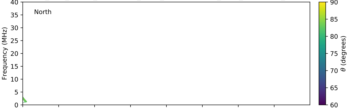
expres_juno_jupiter_ganymede_isaac_lossc-wid1deg_3kev_20170407_v01.cdf
