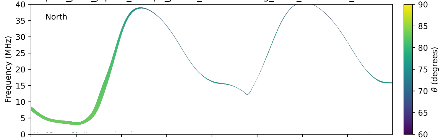
expres_juno_jupiter_europa_jrm09_lossc-wid1deg_3kev_20170426_v01.cdf
