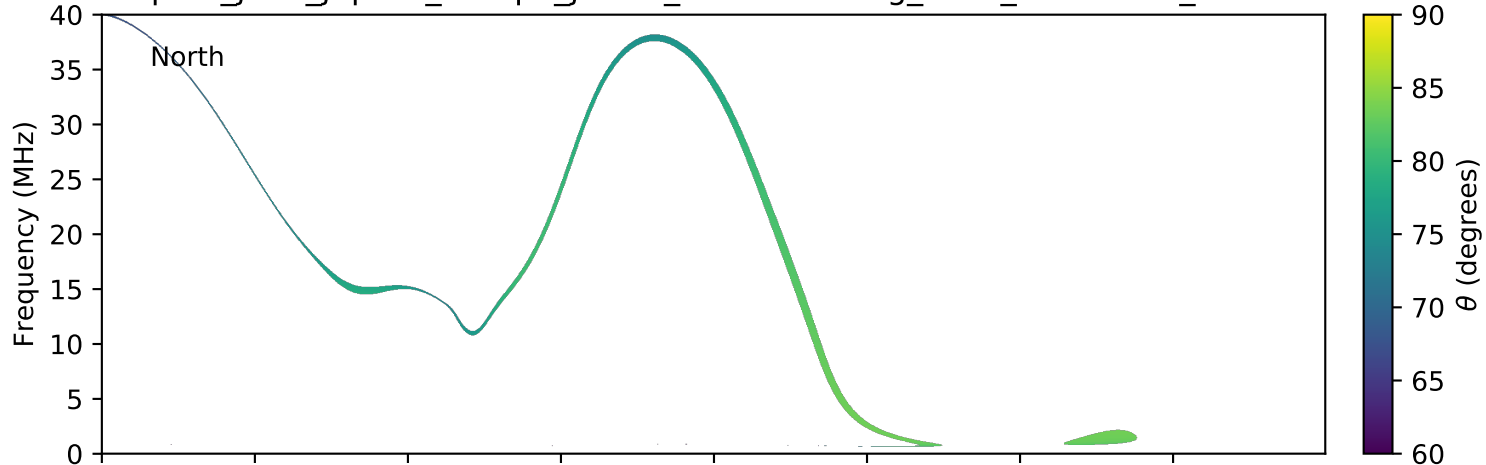
expres_juno_jupiter_europa_jrm09_lossc-wid1deg_3kev_20170416_v01.cdf
