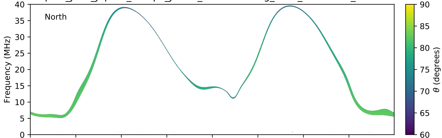
expres_juno_jupiter_europa_jrm09_lossc-wid1deg_3kev_20170412_v01.cdf
