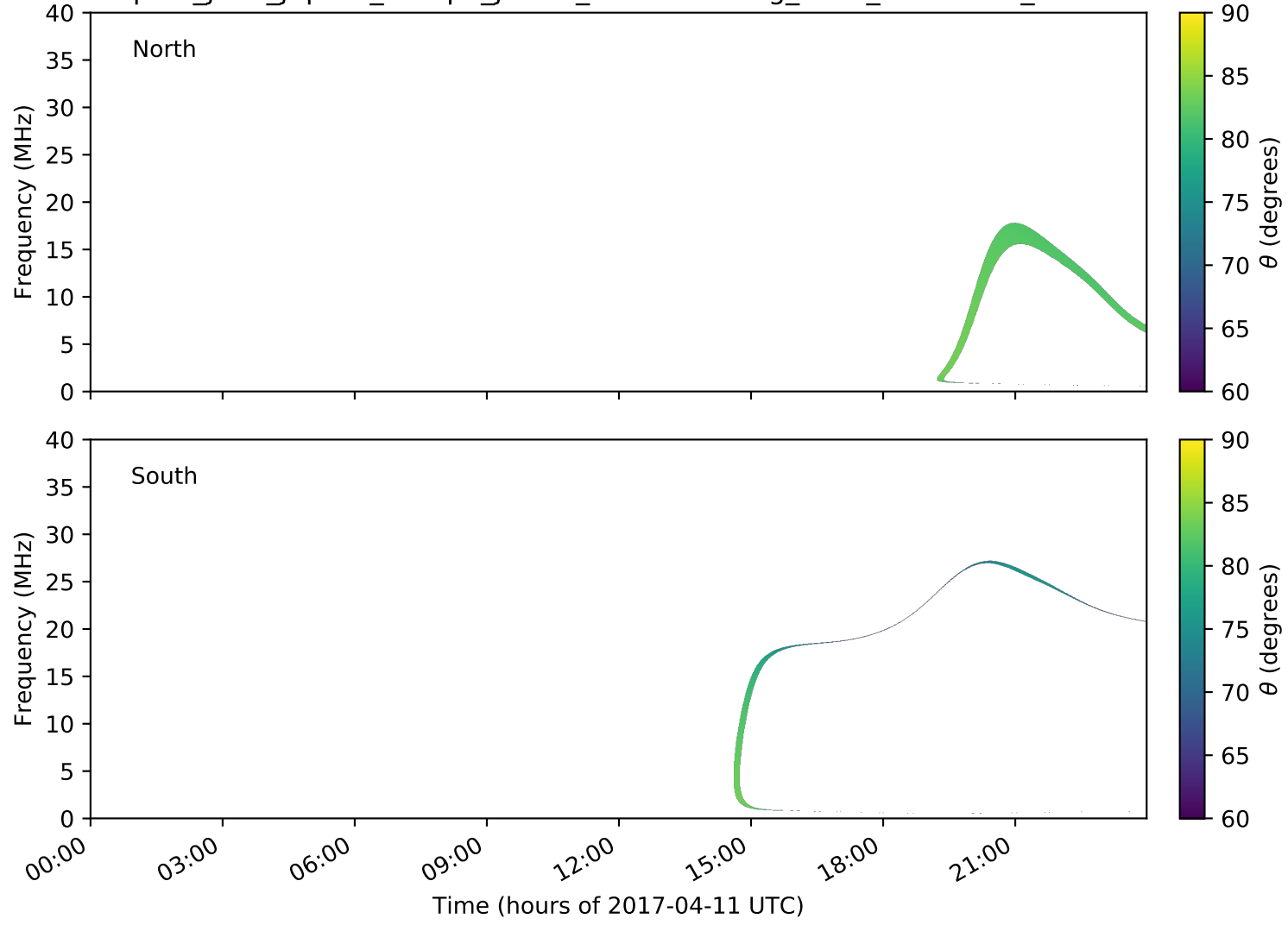
expres_juno_jupiter_europa_jrm09_lossc-wid1deg_3kev_20170411_v01.cdf
