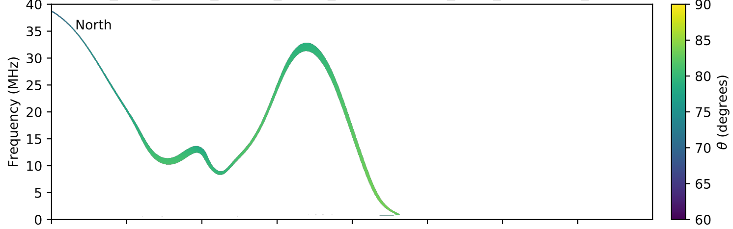
expres_juno_jupiter_europa_jrm09_lossc-wid1deg_3kev_20170409_v01.cdf
