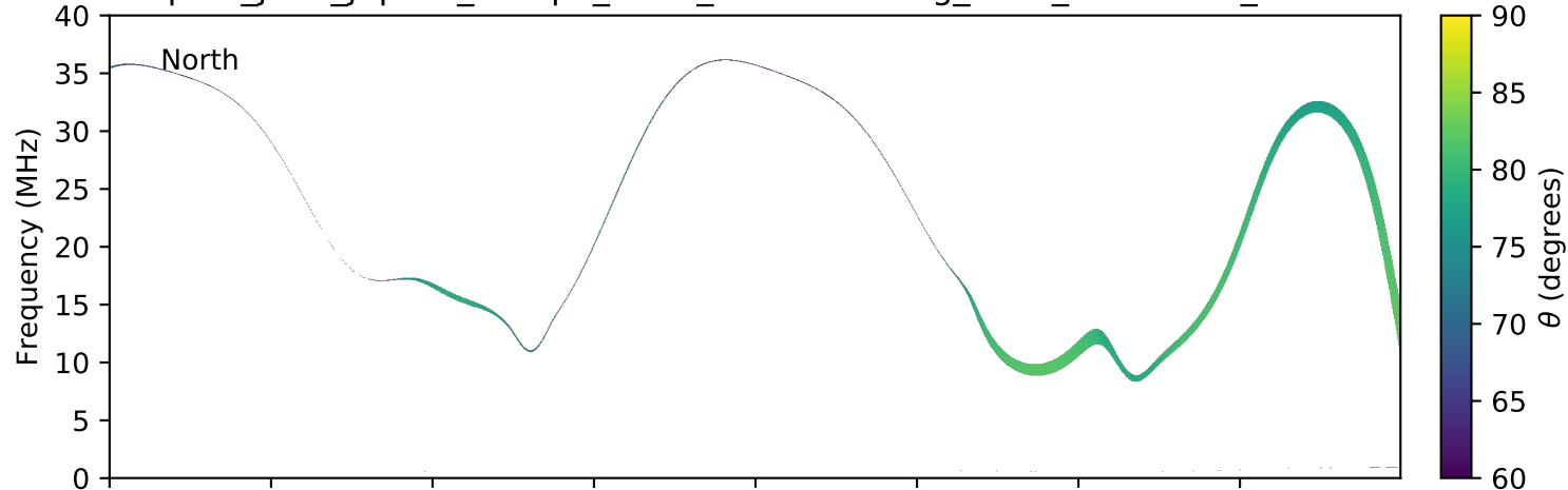
expres_juno_jupiter_europa_isaac_lossc-wid1deg_3kev_20170430_v01.cdf
