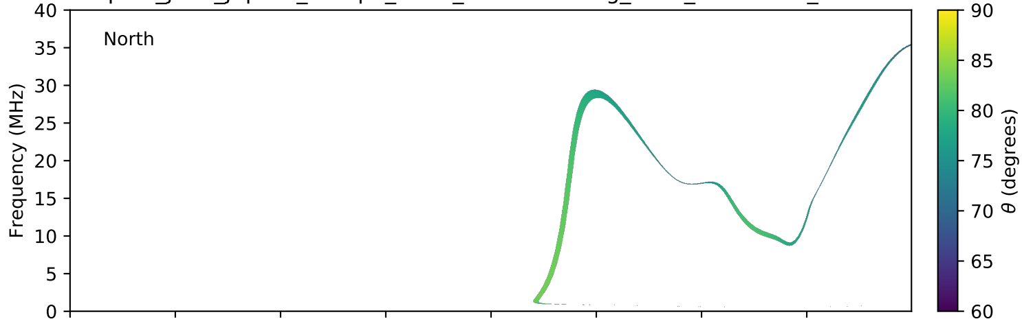
expres_juno_jupiter_europa_isaac_lossc-wid1deg_3kev_20170429_v01.cdf
