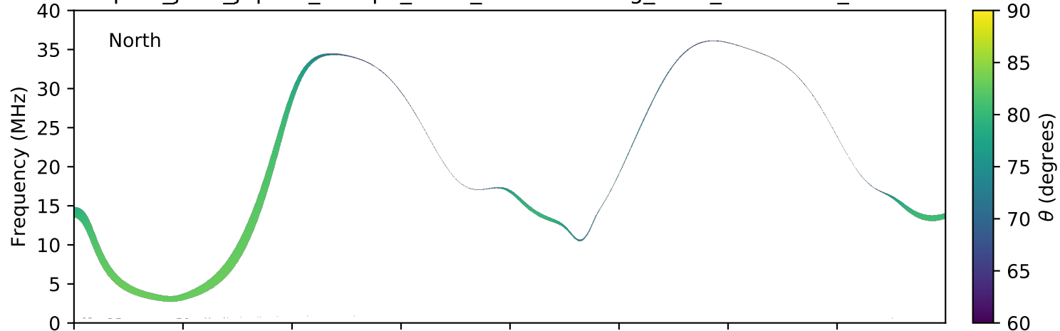
expres_juno_jupiter_europa_isaac_lossc-wid1deg_3kev_20170426_v01.cdf
