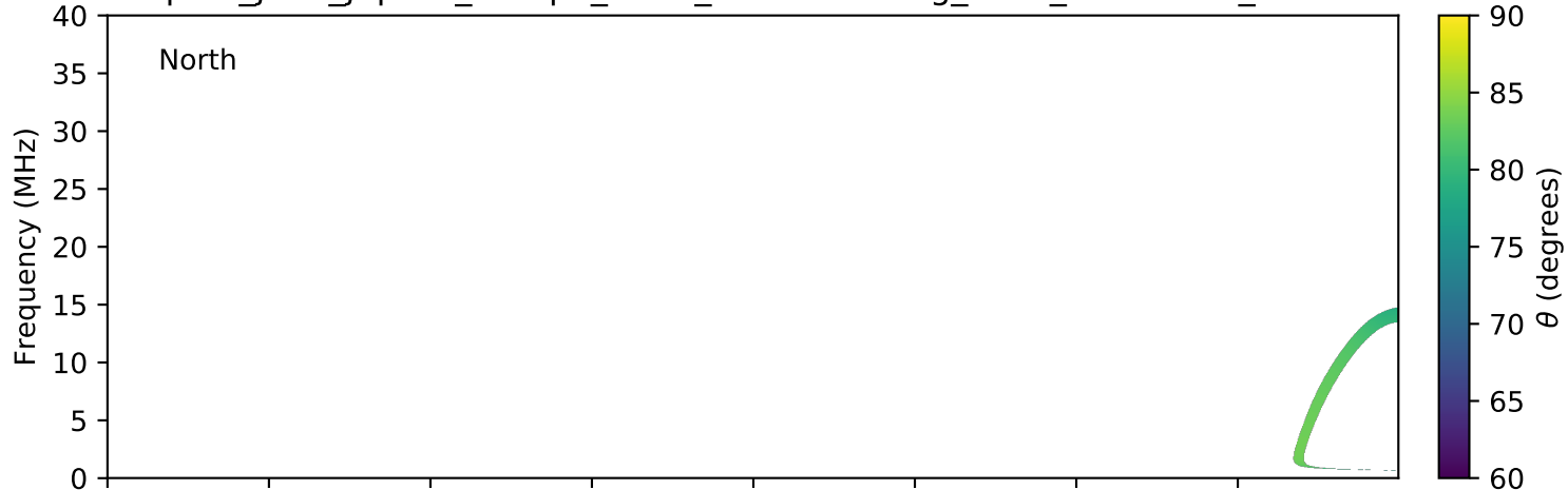
expres_juno_jupiter_europa_isaac_lossc-wid1deg_3kev_20170425_v01.cdf
