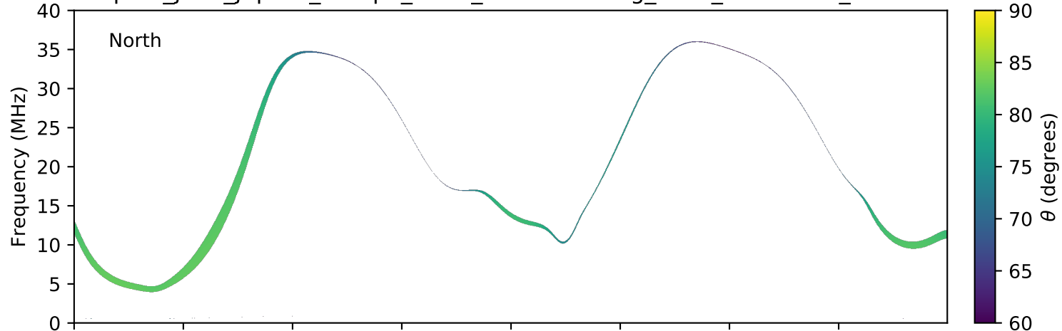
expres_juno_jupiter_europa_isaac_lossc-wid1deg_3kev_20170419_v01.cdf
