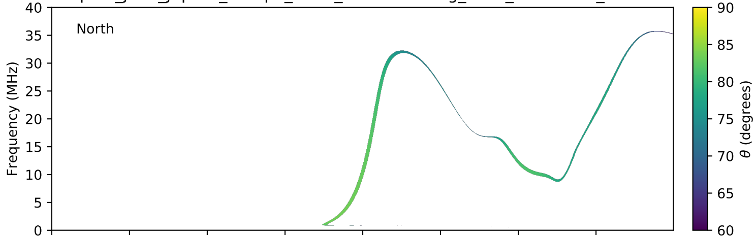
expres_juno_jupiter_europa_isaac_lossc-wid1deg_3kev_20170415_v01.cdf
