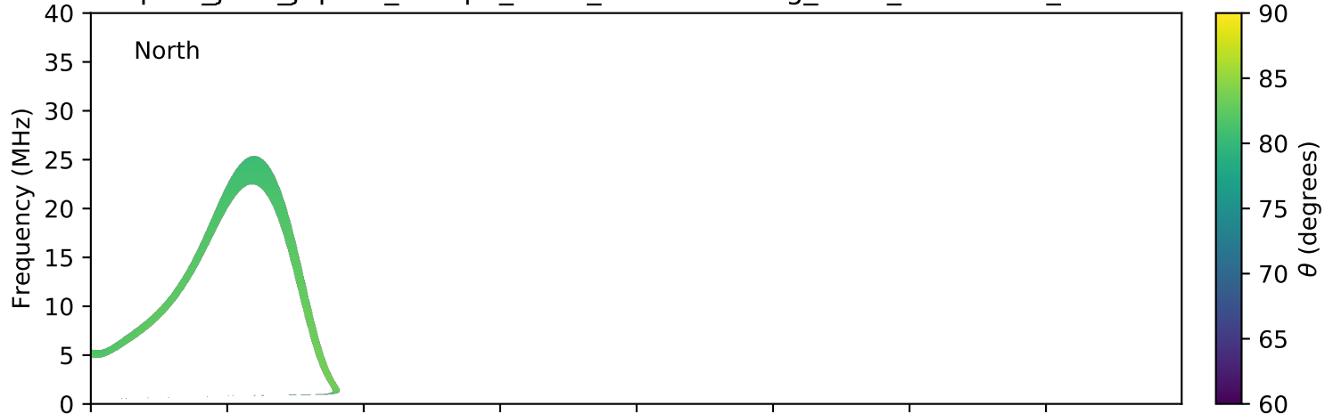
expres_juno_jupiter_europa_isaac_lossc-wid1deg_3kev_20170413_v01.cdf
