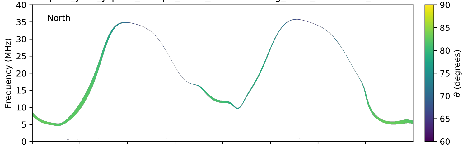
expres_juno_jupiter_europa_isaac_lossc-wid1deg_3kev_20170412_v01.cdf
