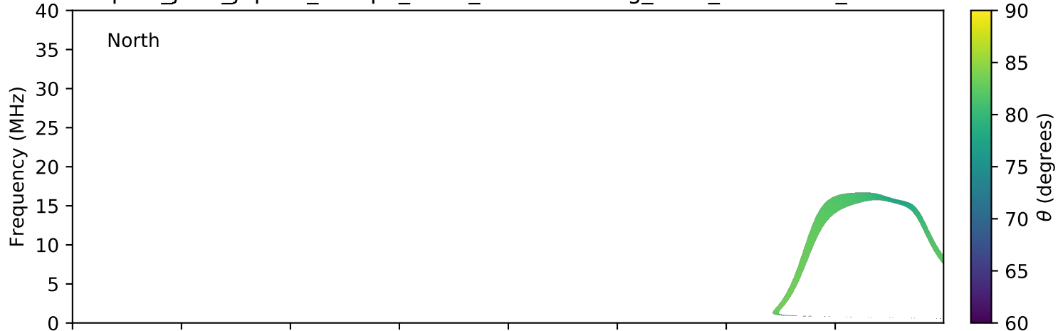
expres_juno_jupiter_europa_isaac_lossc-wid1deg_3kev_20170411_v01.cdf
