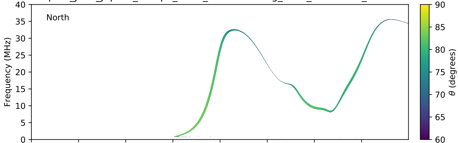
expres_juno_jupiter_europa_isaac_lossc-wid1deg_3kev_20170408_v01.cdf
