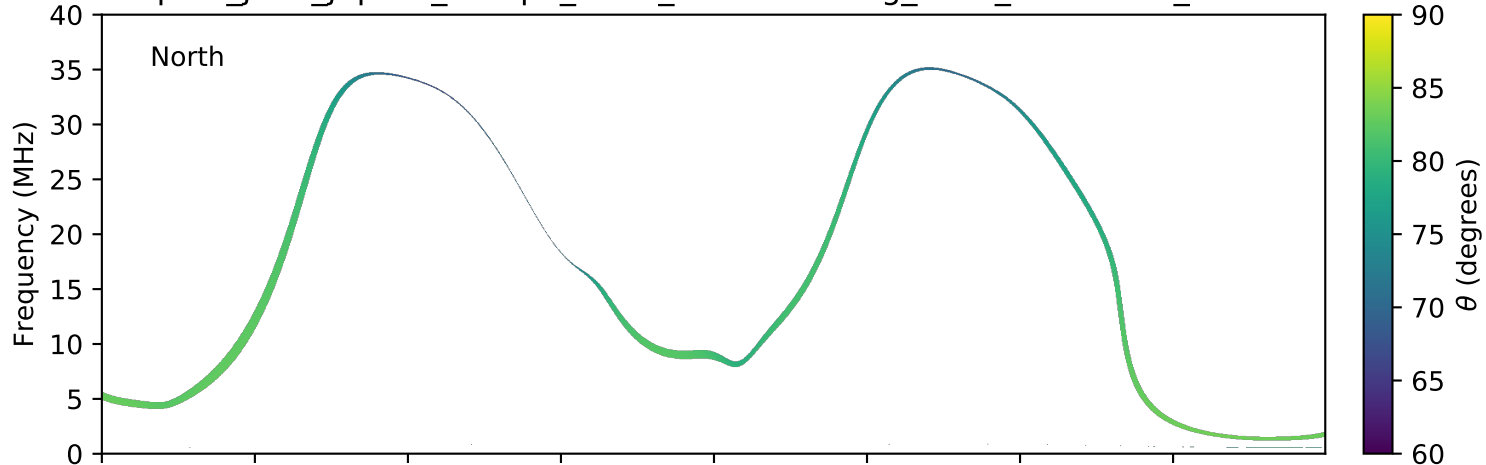
expres_juno_jupiter_europa_isaac_lossc-wid1deg_3kev_20170405_v01.cdf
