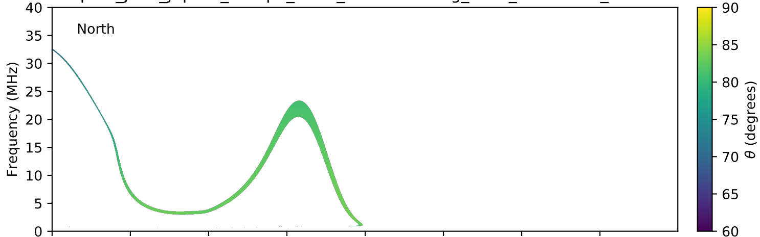
expres_juno_jupiter_europa_isaac_lossc-wid1deg_3kev_20170402_v01.cdf
