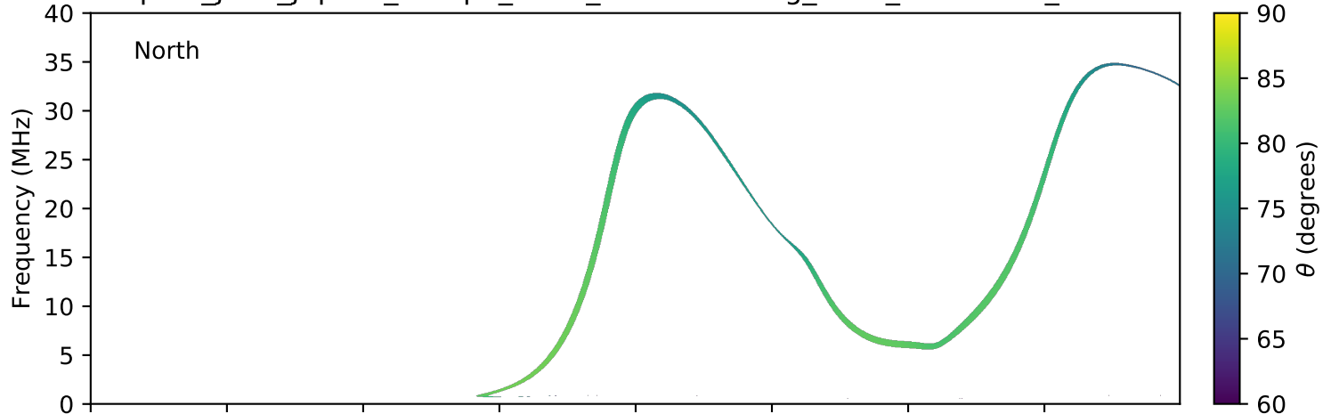
expres_juno_jupiter_europa_isaac_lossc-wid1deg_3kev_20170401_v01.cdf
