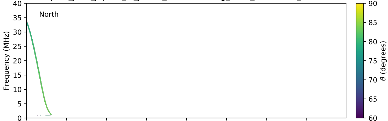
expres_juno_jupiter_io_jrm09_lossc-wid1deg_3kev_20170223_v01.cdf
