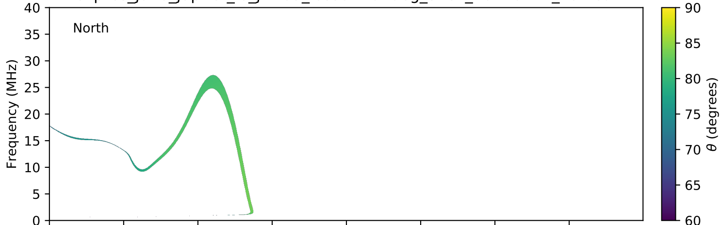
expres_juno_jupiter_io_jrm09_lossc-wid1deg_3kev_20170221_v01.cdf
