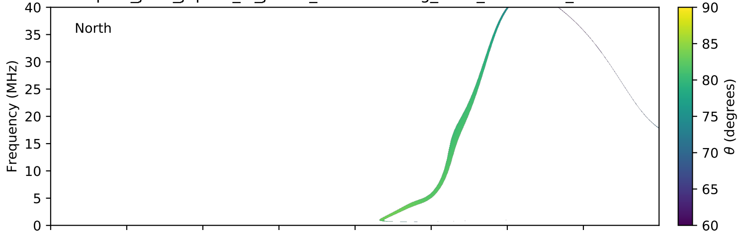
expres_juno_jupiter_io_jrm09_lossc-wid1deg_3kev_20170220_v01.cdf
