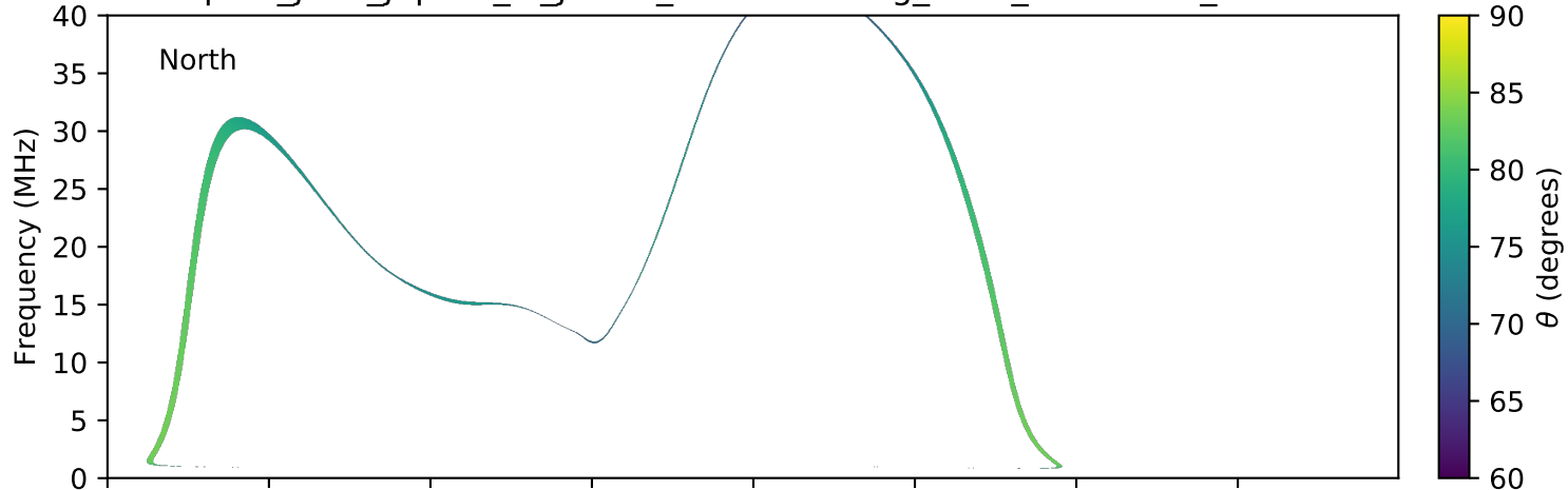
expres_juno_jupiter_io_jrm09_lossc-wid1deg_3kev_20170217_v01.cdf
