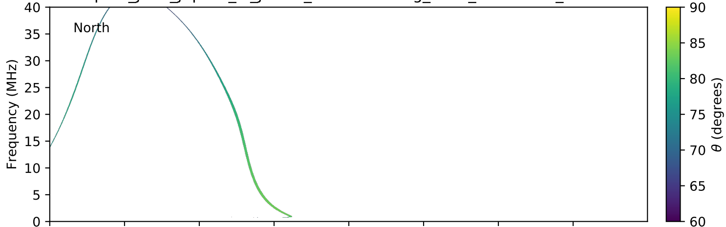
expres_juno_jupiter_io_jrm09_lossc-wid1deg_3kev_20170212_v01.cdf
