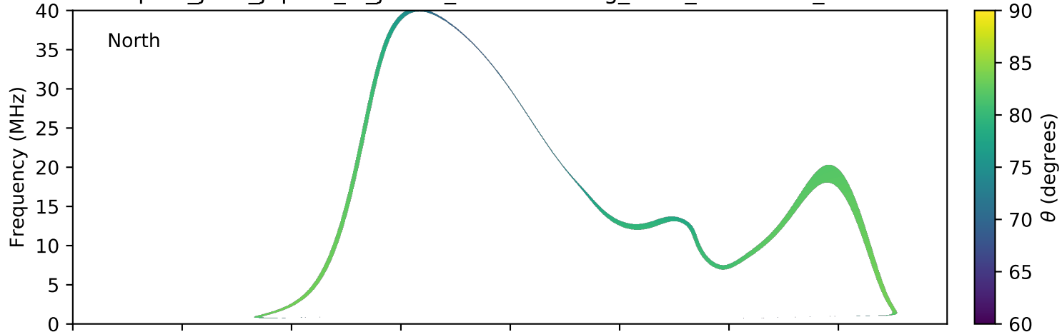
expres_juno_jupiter_io_jrm09_lossc-wid1deg_3kev_20170208_v01.cdf
