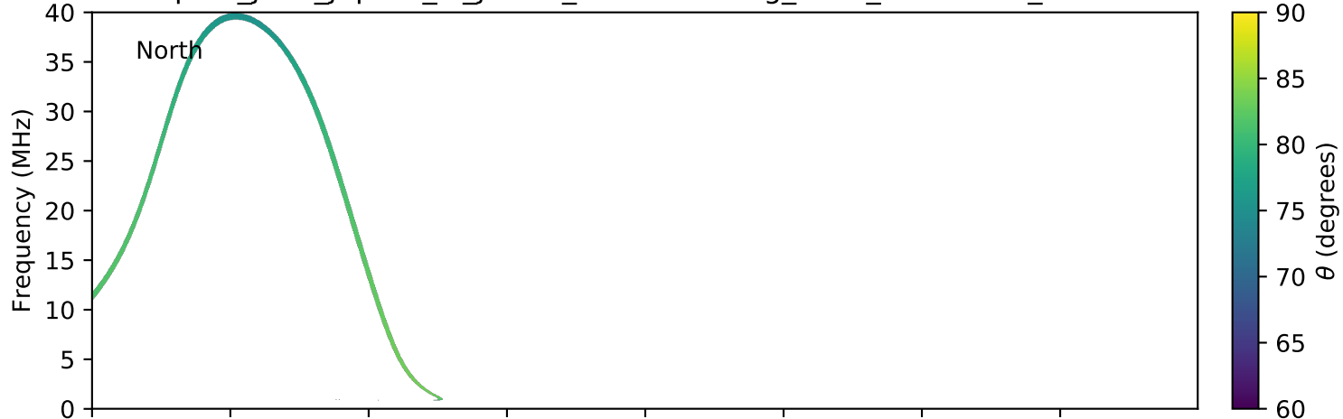
expres_juno_jupiter_io_jrm09_lossc-wid1deg_3kev_20170205_v01.cdf
