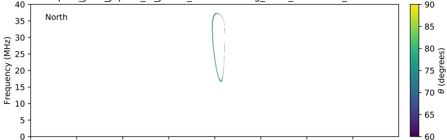
expres_juno_jupiter_io_jrm09_lossc-wid1deg_3kev_20170202_v01.cdf
