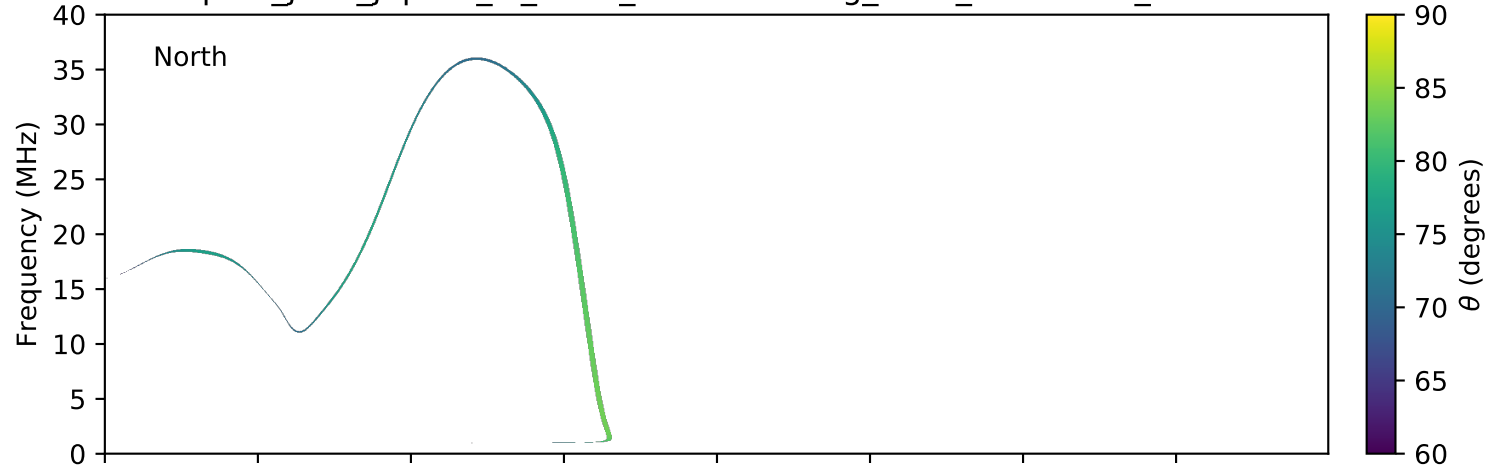
expres_juno_jupiter_io_isaac_lossc-wid1deg_3kev_20170228_v01.cdf
