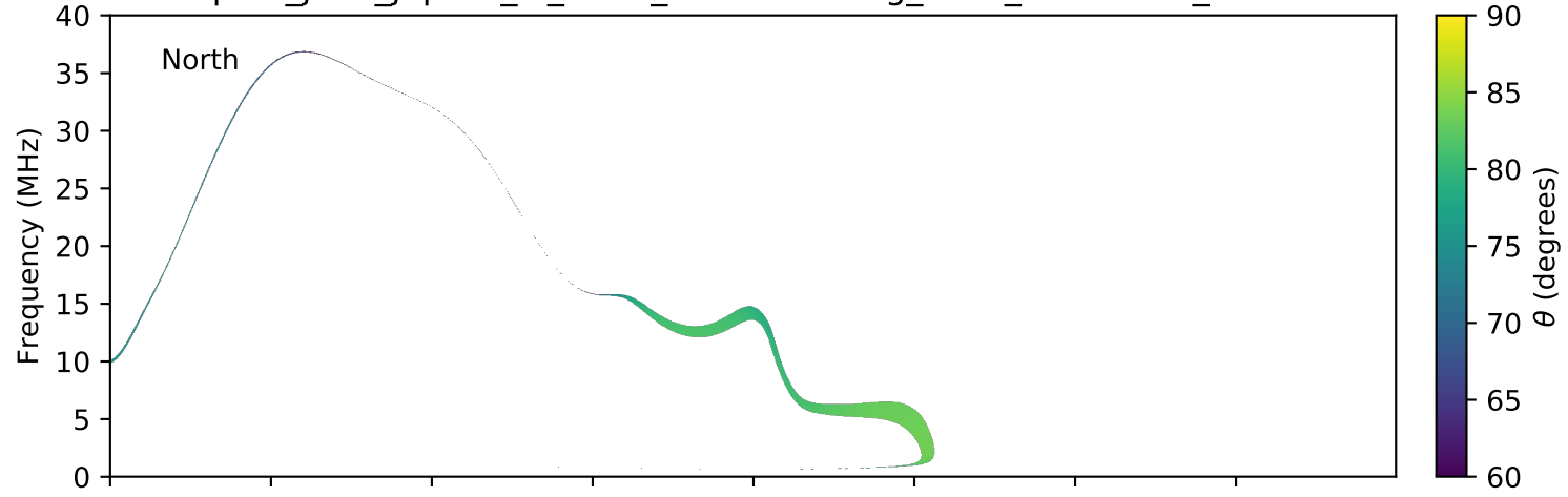
expres_juno_jupiter_io_isaac_lossc-wid1deg_3kev_20170226_v01.cdf
