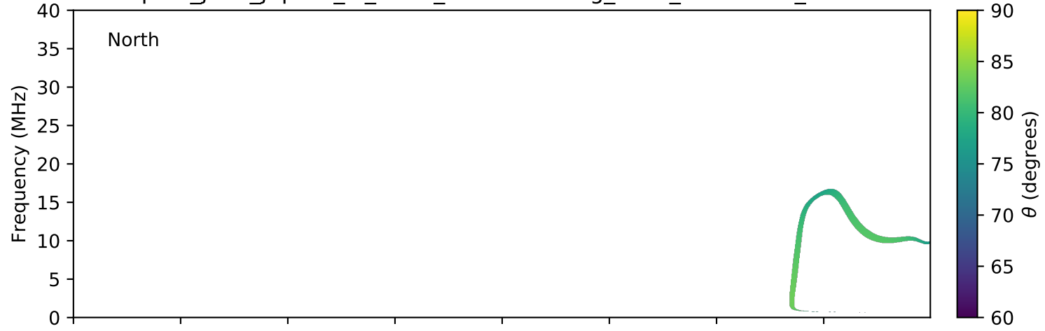
expres_juno_jupiter_io_isaac_lossc-wid1deg_3kev_20170225_v01.cdf
