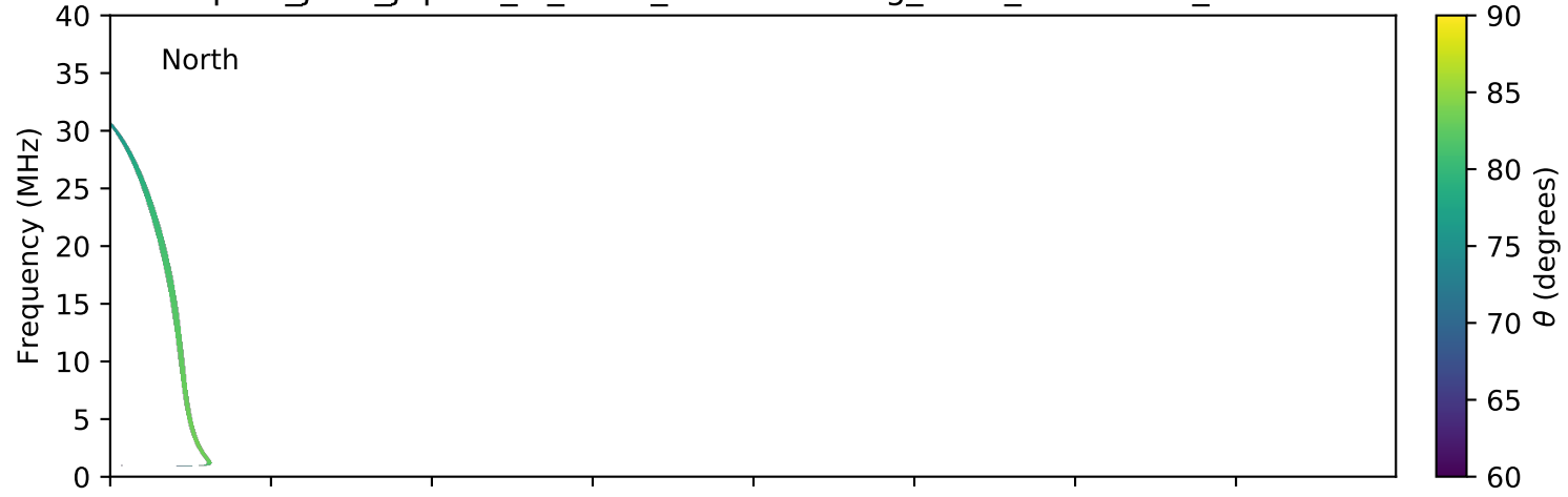
expres_juno_jupiter_io_isaac_lossc-wid1deg_3kev_20170223_v01.cdf
