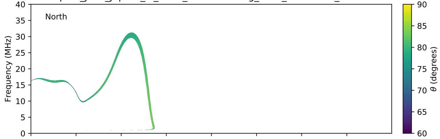
expres_juno_jupiter_io_isaac_lossc-wid1deg_3kev_20170221_v01.cdf
