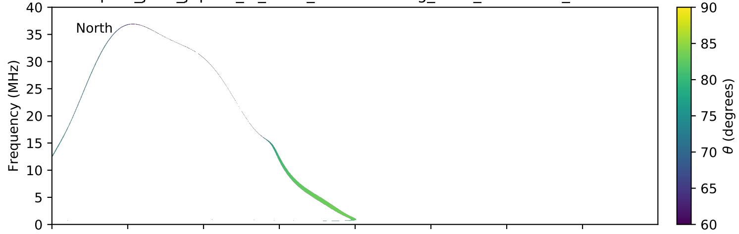
expres_juno_jupiter_io_isaac_lossc-wid1deg_3kev_20170219_v01.cdf
