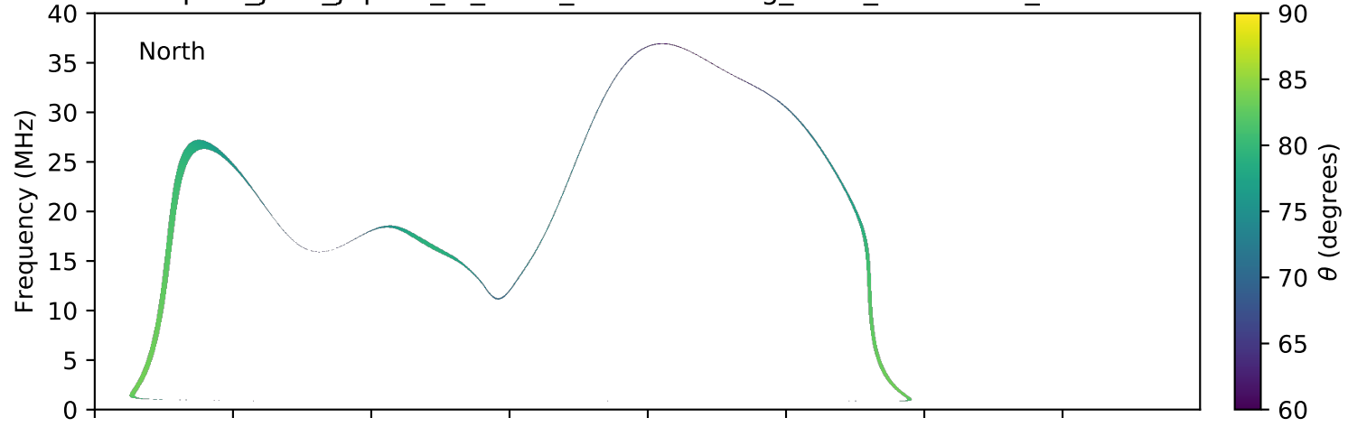
expres_juno_jupiter_io_isaac_lossc-wid1deg_3kev_20170217_v01.cdf
