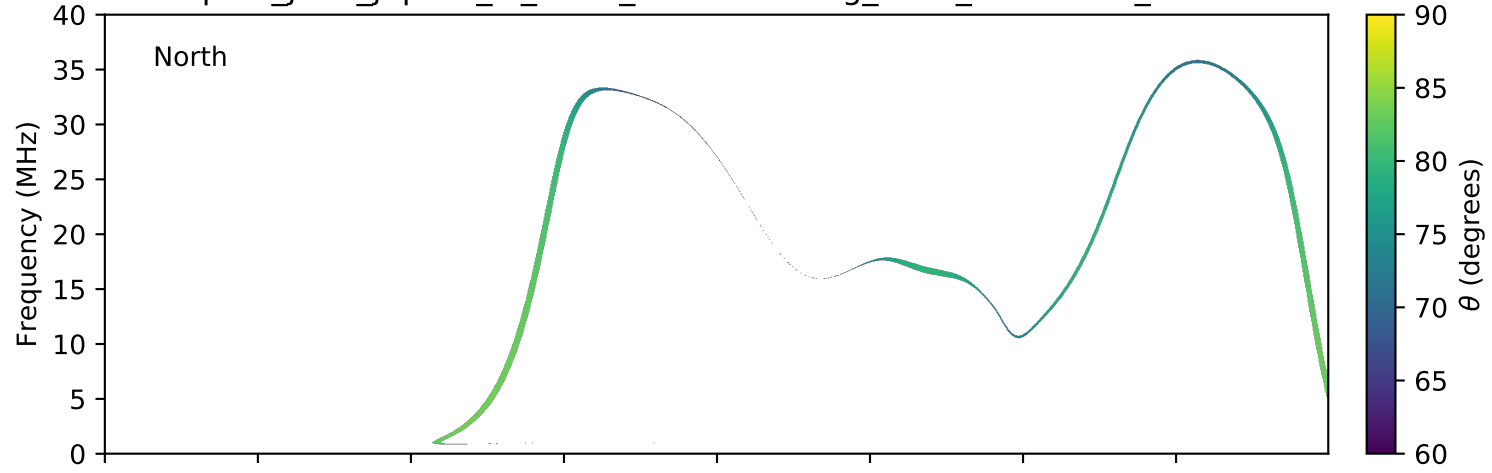
expres_juno_jupiter_io_isaac_lossc-wid1deg_3kev_20170215_v01.cdf
