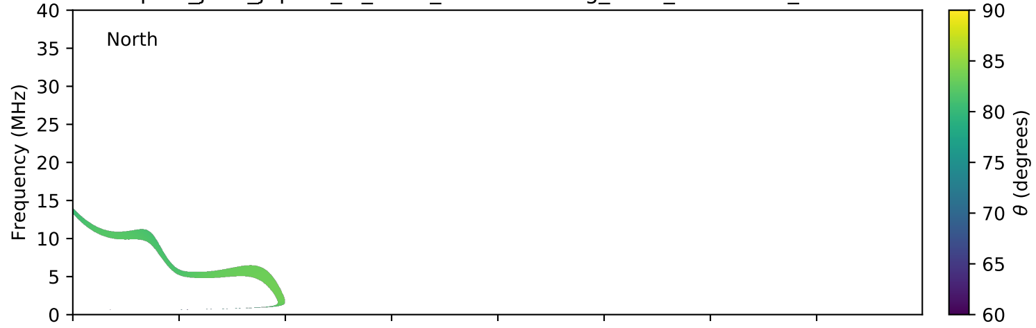
expres_juno_jupiter_io_isaac_lossc-wid1deg_3kev_20170214_v01.cdf
