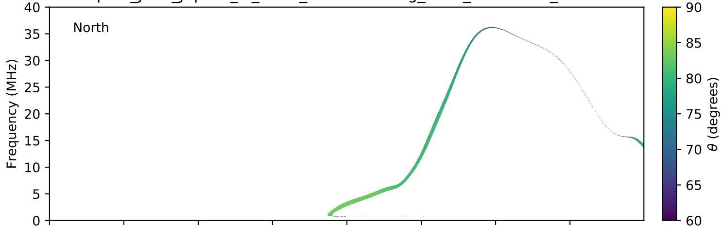
expres_juno_jupiter_io_isaac_lossc-wid1deg_3kev_20170213_v01.cdf
