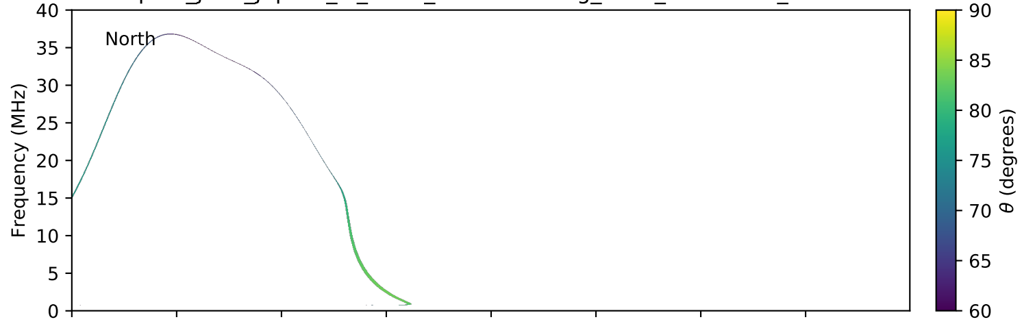
expres_juno_jupiter_io_isaac_lossc-wid1deg_3kev_20170212_v01.cdf
