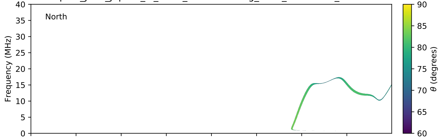
expres_juno_jupiter_io_isaac_lossc-wid1deg_3kev_20170211_v01.cdf
