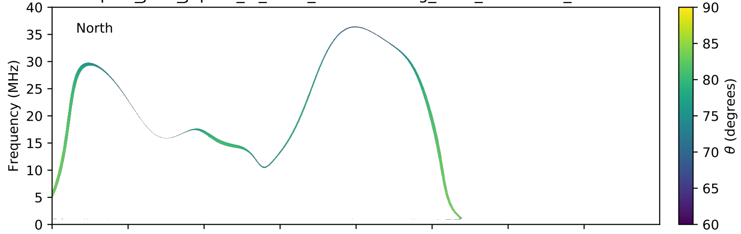
expres_juno_jupiter_io_isaac_lossc-wid1deg_3kev_20170210_v01.cdf
