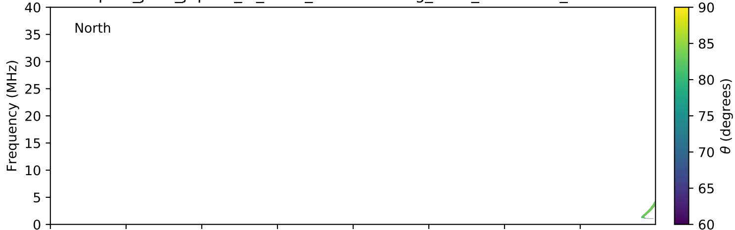
expres_juno_jupiter_io_isaac_lossc-wid1deg_3kev_20170209_v01.cdf
