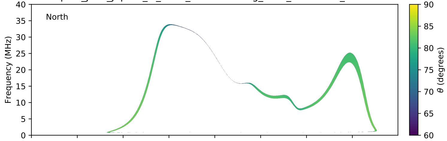
expres_juno_jupiter_io_isaac_lossc-wid1deg_3kev_20170208_v01.cdf
