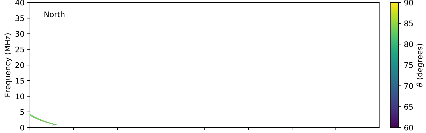
expres_juno_jupiter_io_isaac_lossc-wid1deg_3kev_20170207_v01.cdf
